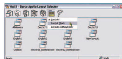
Layout Selector allows to view the stack of loaded layouts on a display wall
